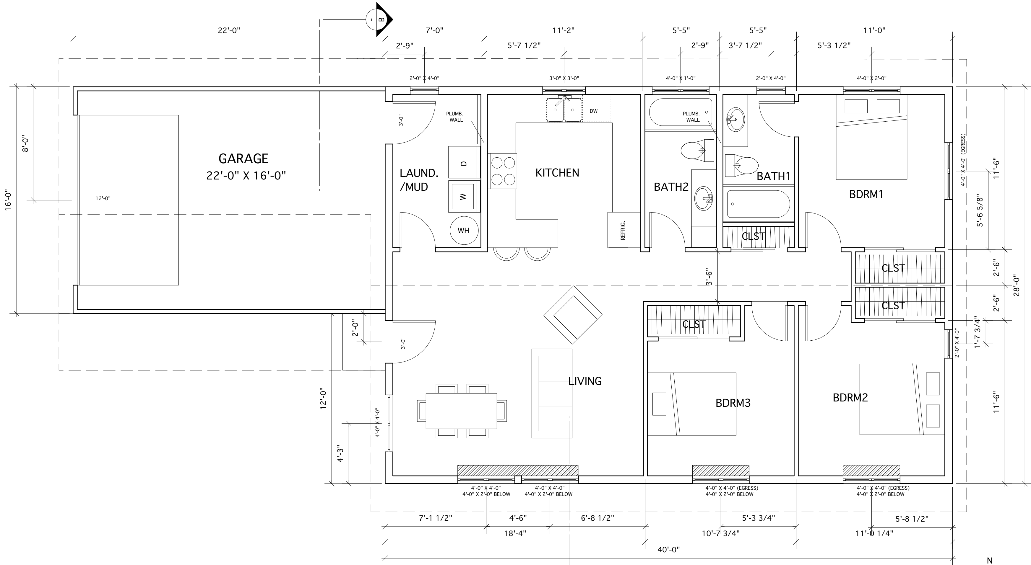
PLAN VIEW- PH3A & 3D, LOT #4 & PH3C Scale: 1/4" = 1'-0" 1120 SQFT- (3)BEDROOM, (2)BATH
